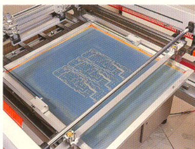
Screen insertion & holding
